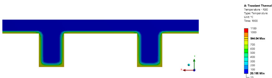
Figure 6 – Temperature profiles of TCC slab after 30 minutes of standard ISO 834 fire [14]
